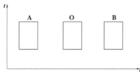
Fig. 1. A space-time diagram of space-like separated regions A , B , and O . Sending signals from O to A \cup B is considered.
